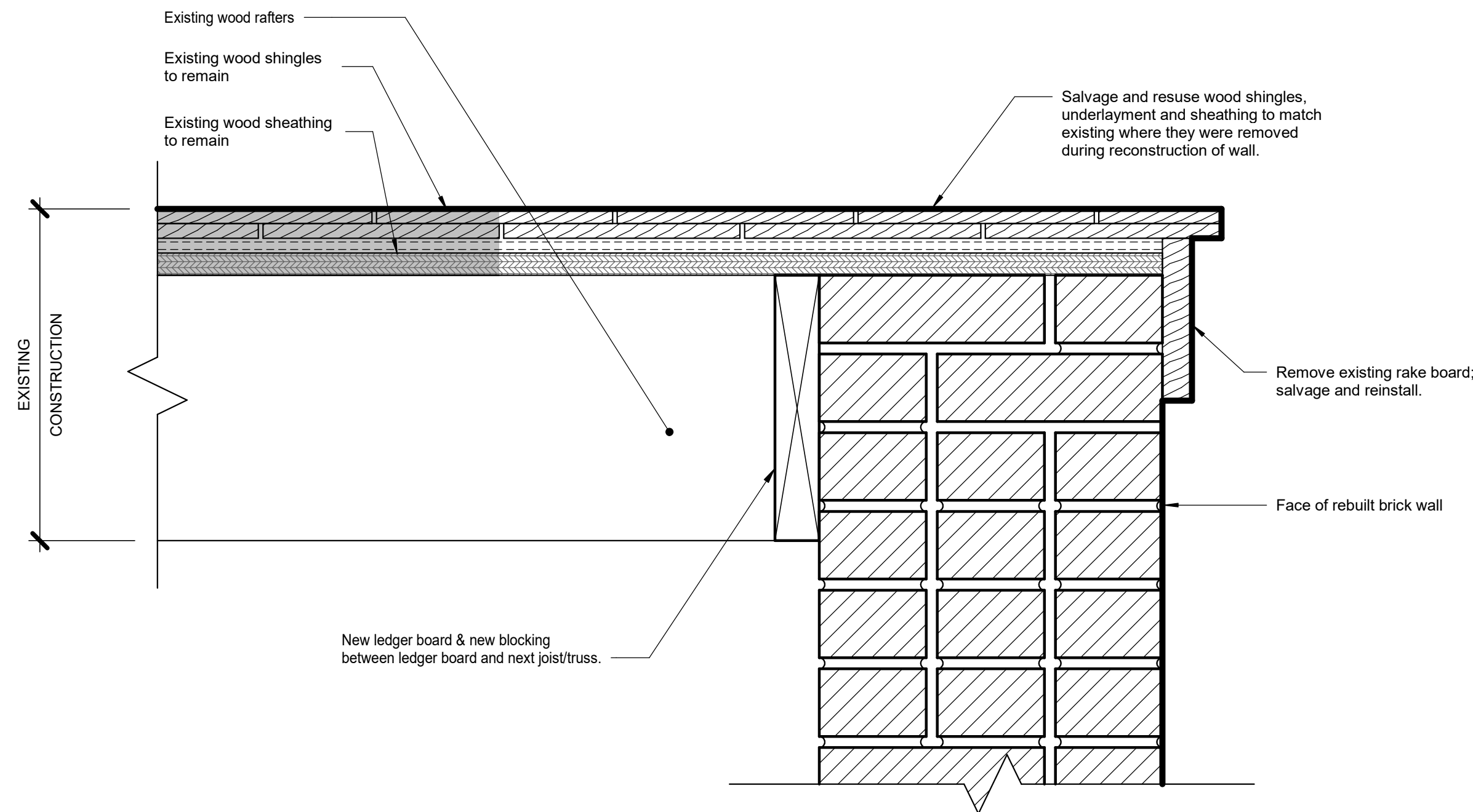
1 Roof Edge Detail at Eaves 3" = 1'-0"
