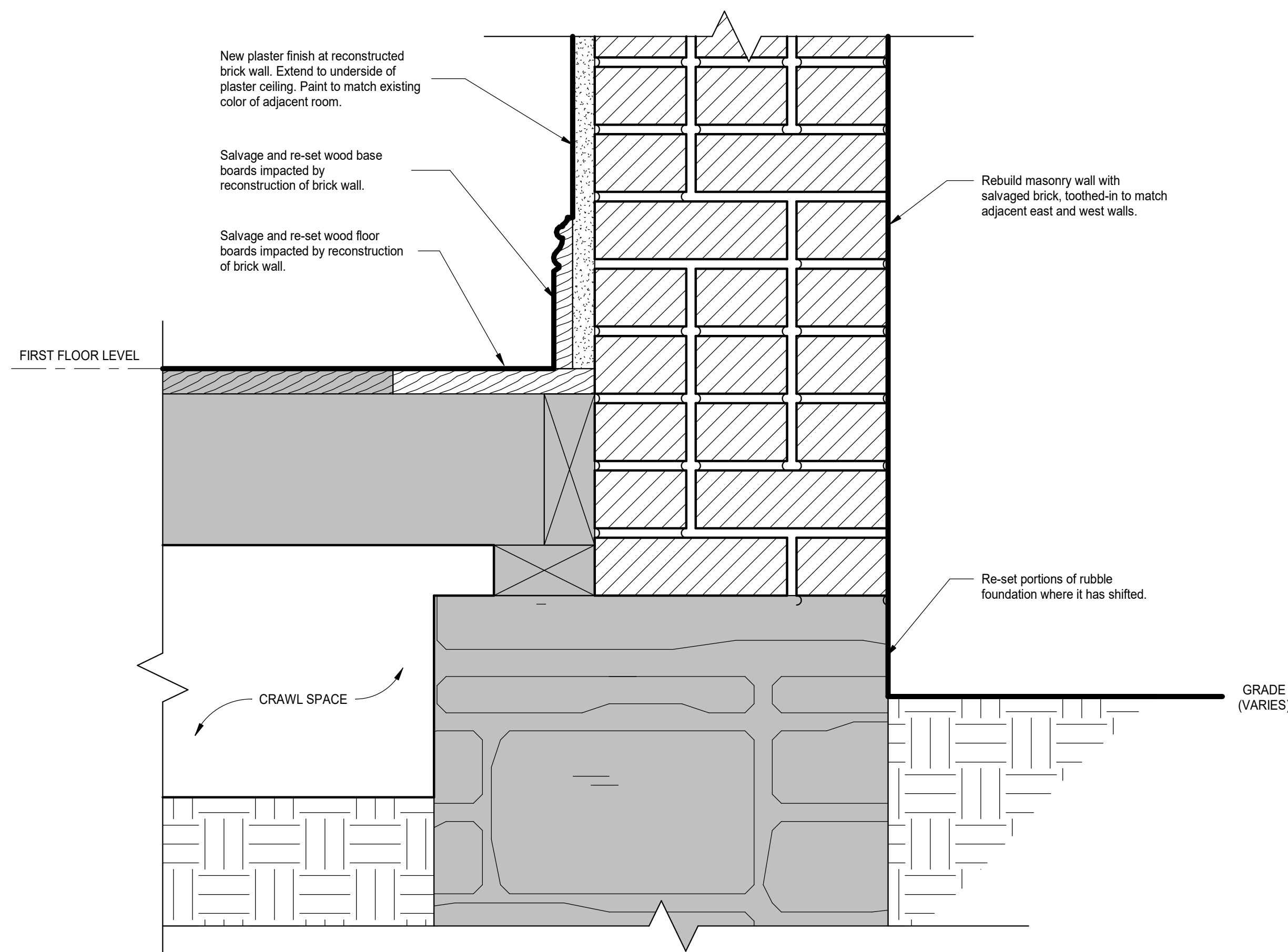
3 Wall Section - Sill Detail 3" = 1'-0"
