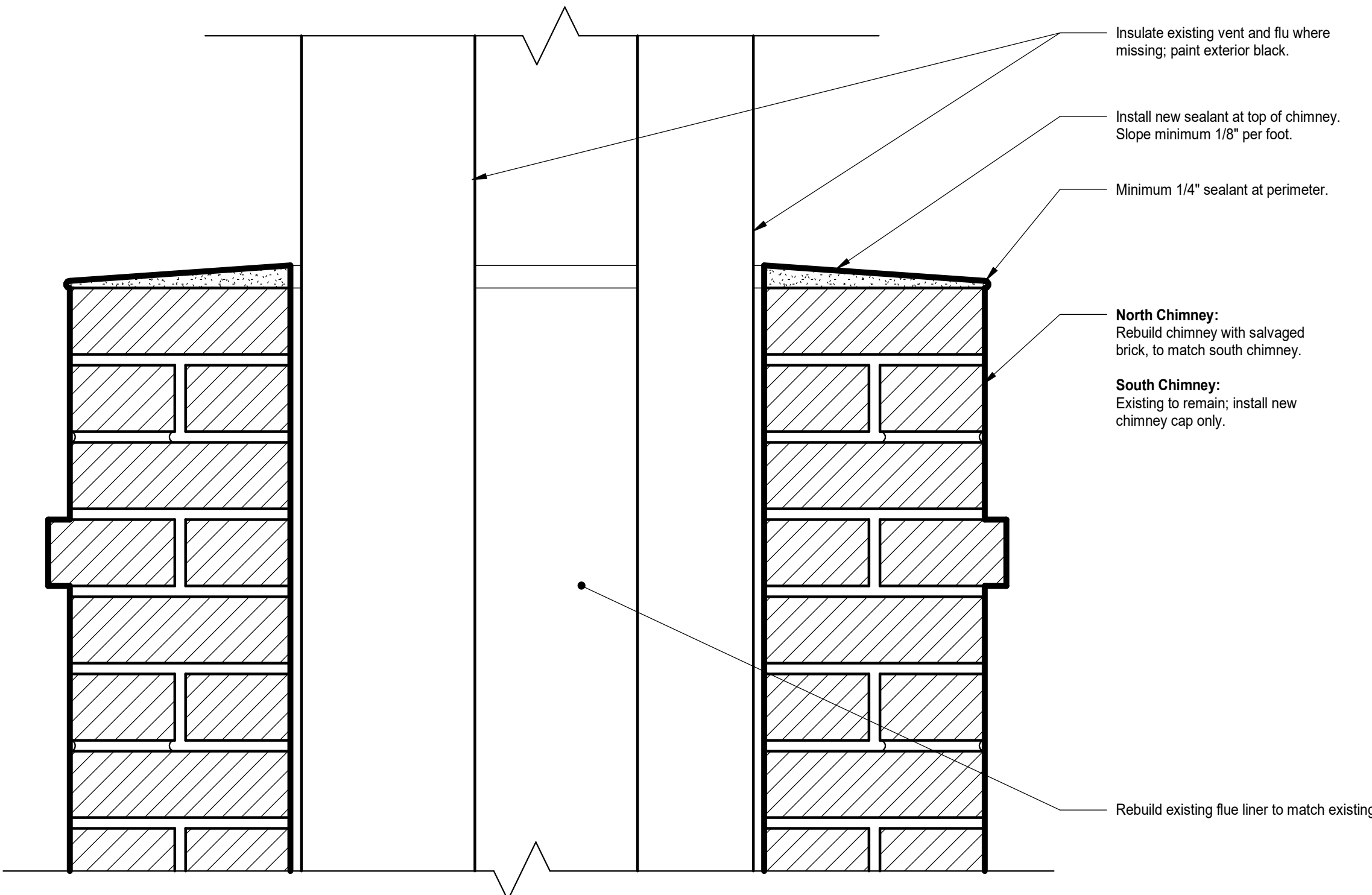
4 Chimney Cap - Section 3" = 1'-0"
