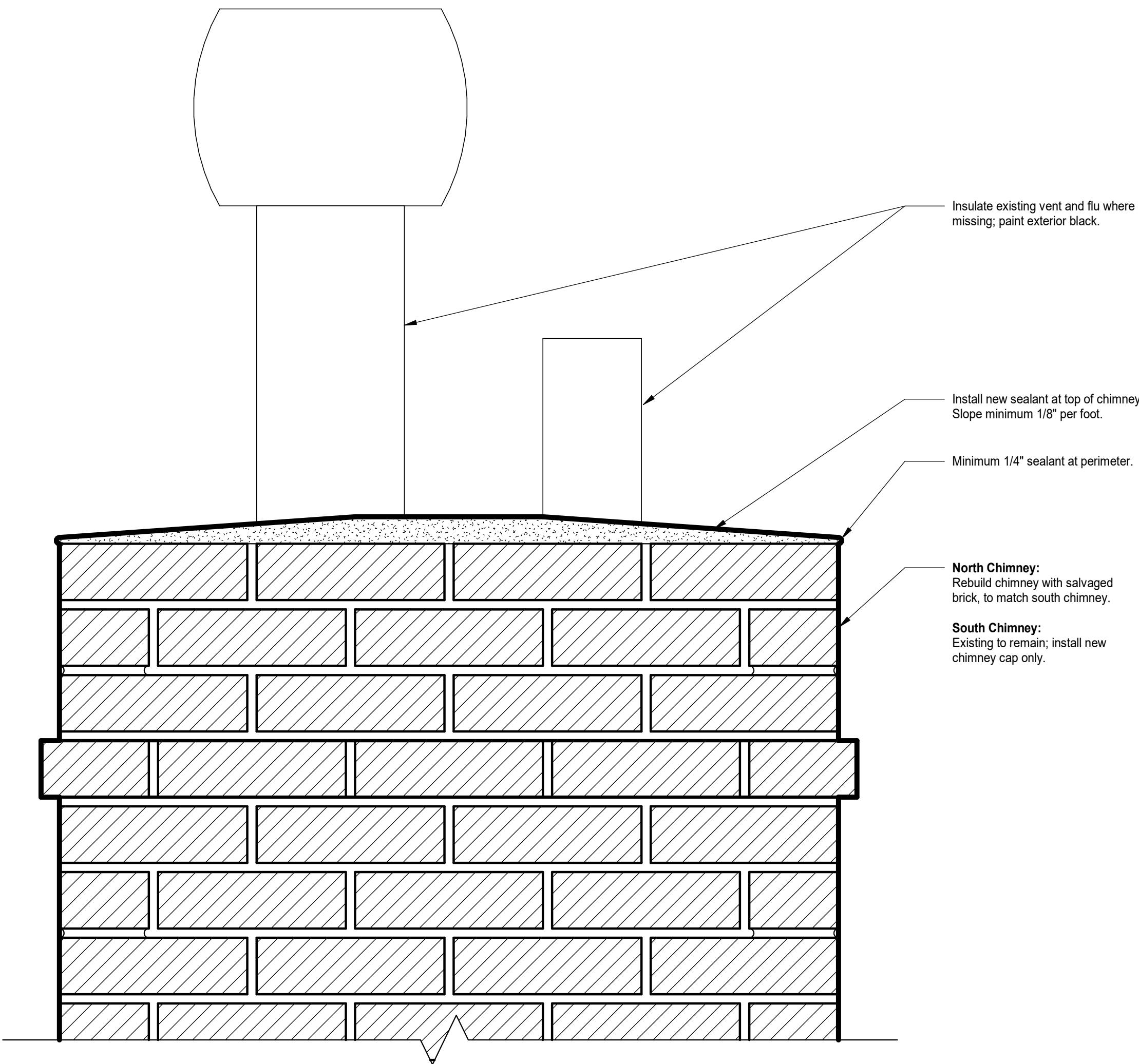
2 Chimney Cap - Elevation 3" = 1'-0"
