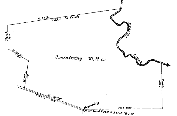
4 DIAGRAM Showing fractional part of Section described by Miles and Bounds.
