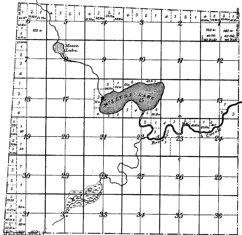
2 DIAGRAM Showing Official Plat of a Township Sectionized and Numbered by Government Surveyors with the fractions on North and West side of Township with plan of numbering fractional lots where bounded by Lake or Creek.
